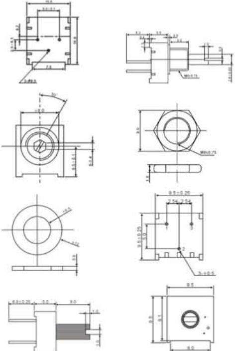
RKT -3386F,K,P,R,U,Y-EY5 (RESISTANCE CODE)-L
