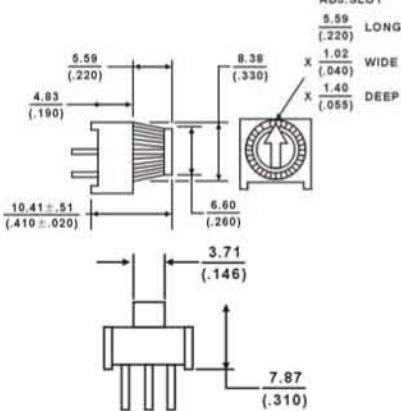
RKT -3386F,K,P,R,U,Y-EY5 (RESISTANCE CODE)-L
