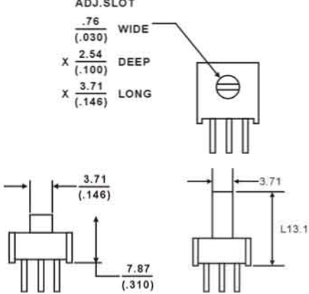
RKT -3386(STYLE)-EY5-(RESISTANCE CODE)-T
